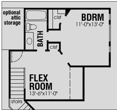
Guest Suite Layout ± 449 Square Feet
