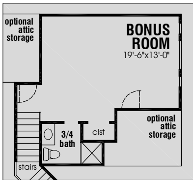
Bonus Room with 3/4 Bath ± 419 Square Feet
