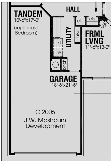
Tandem Garage, Formal Living adds 6'-4" to total depth
